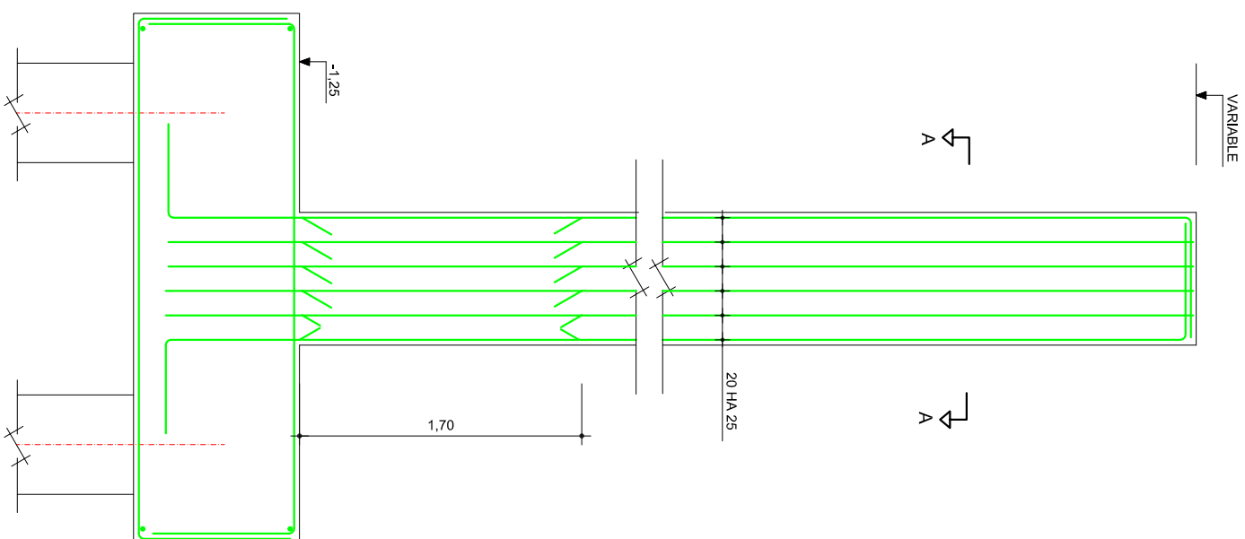
COUPÉ POTEAUX TYPE - 2 ESCALA 1:20
